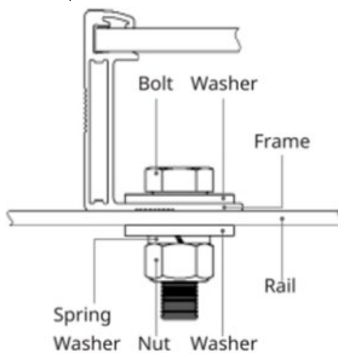
Figure 1 Screw installation
