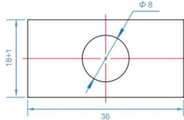
Figure 6 Special rectangular washer
