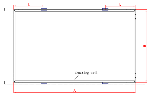
Drawing 2: Mounting rail parallel the long side
