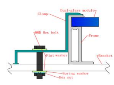
Figure 6 Single-side clamp installation
