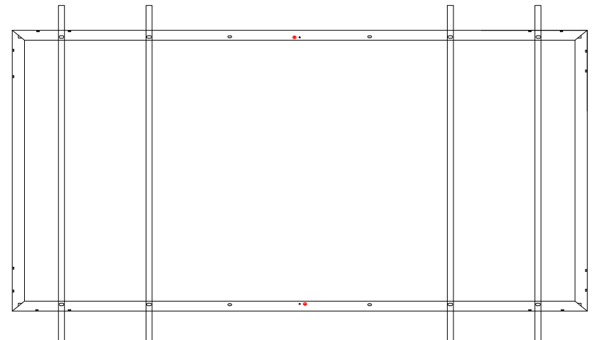
(8 mounting holes for 166 modules and 182-BMB)
