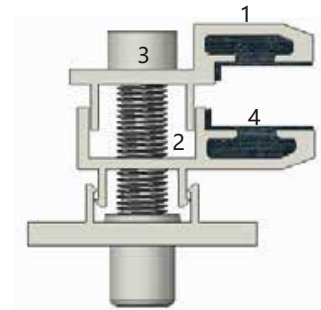
Figure 2 Single-side clamp
