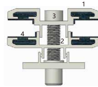
Figure 1 Double-side clamp
